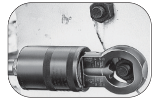
Align mark on cutter blade with scale.
